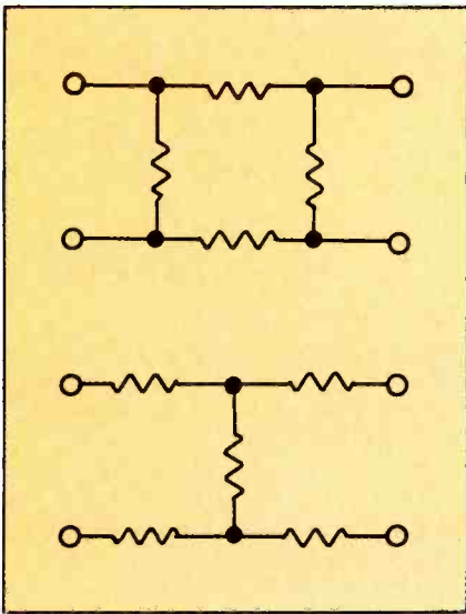
Figure 6. These configurations can be used for impedance matching when you are connecting to balanced transmission lines. They can be obtained directly from the delta- and wye-circuits.
