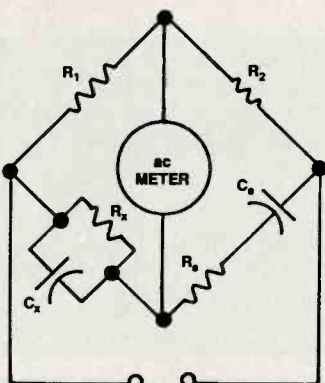
WEIN BRIDGE
