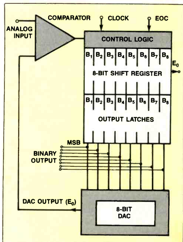
Figure 2. The successive approximation converter makes several successive trials comparing the analog input voltage with a reference generated by a DAC. This circuit consists of a comparator, a control logic section, a shift register, output latches and a DAC.
