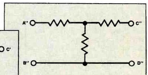
Figure 3. This circuit is sometimes called a Y or wye because of its characteristic shape.
