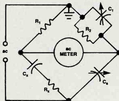
SCHERING BRIDGE
