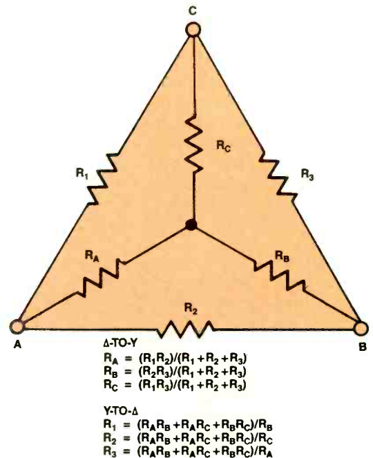
Figure 5. With complicated networks, the delta-wye and wye-delta transform equations can be used to transform configurations and simplify the circuit.
