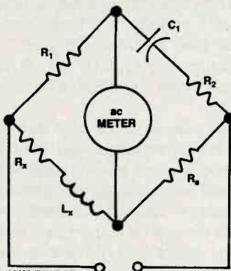
HAY BRIDGE
